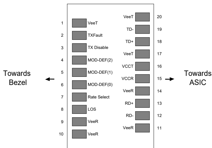
Pinout of Connector Block on Host Board
